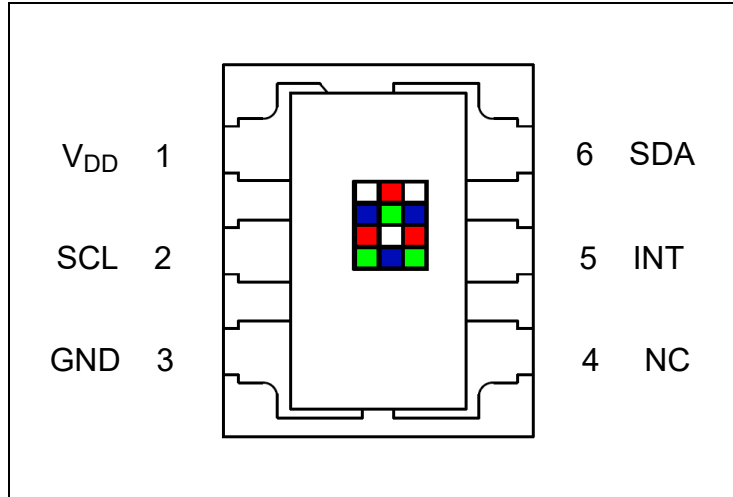
Figure 3: Pin Diagram
